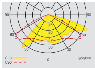
Light distribution curve Outdoor Wall II O CG-S with symmetric optics
