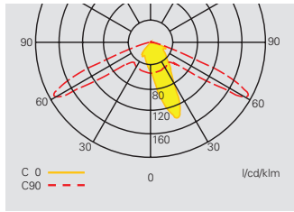
Light distribution curve Outdoor Wall II R CG-S with asymmetric optics
